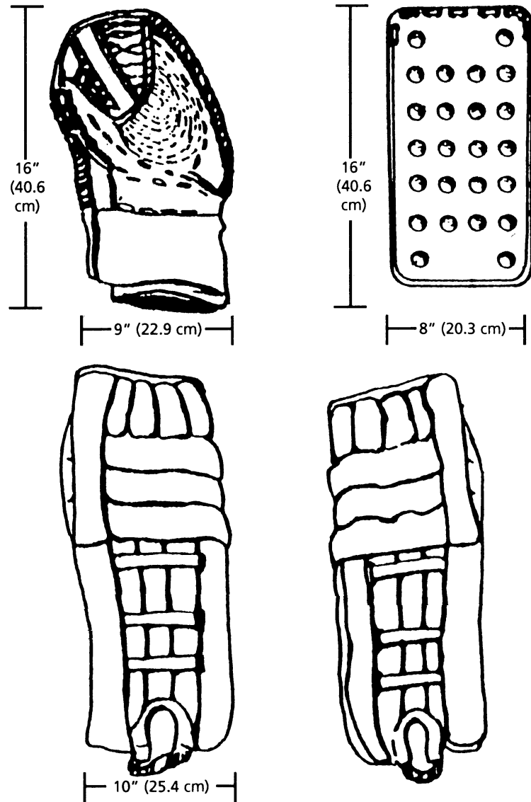
To show measurements only. Refer to Rule 23 - Goalkeepers Equipment.
